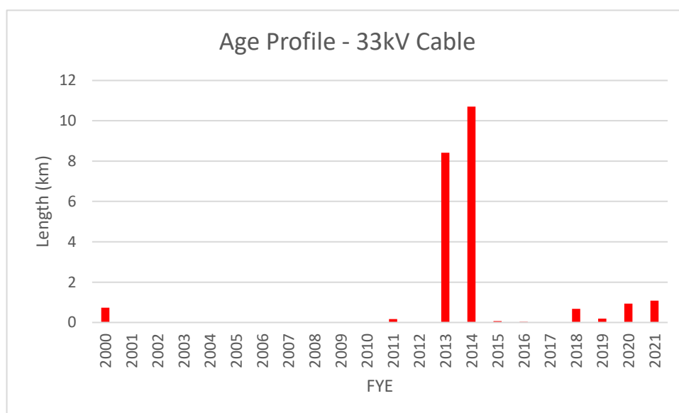
Figure 6.8: Age Profile – 33kV Underground Cable
