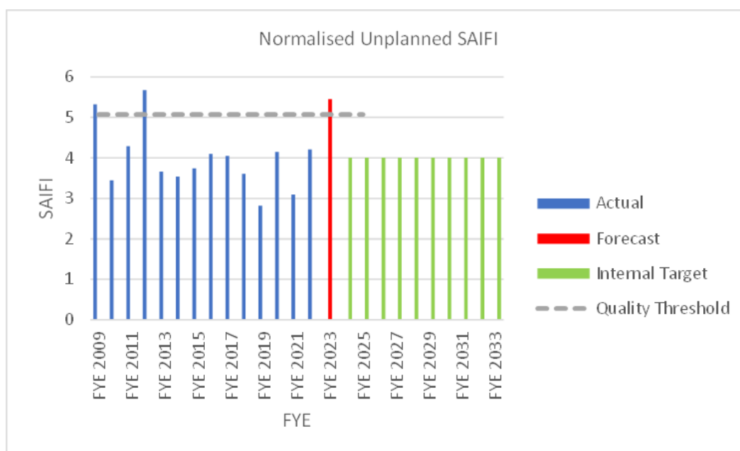
Figure 4.2: Historical and Target Unplanned SAIFI
