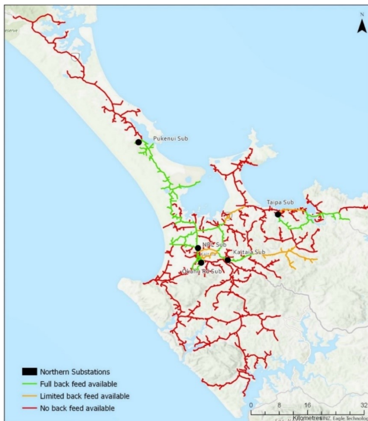
Figure 5.1: Map of Feeder Interconnectivity in the Northern Region
